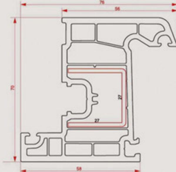
70 mm Pencere Profili 5 Odacıklı 70 mm Window Sash Profile W / 5 Chamber
