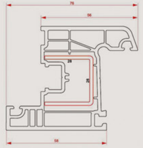
60 mm Pencere Profili 4 Odacıklı 60 mm Window Sash Profile W / 4 Chamber
