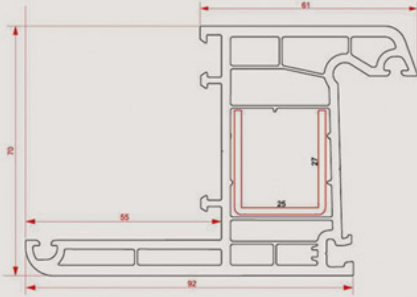
70 mm Pervazlı Kasa Profili 5 Odacıklı 70 mm Wide Frame With Border W / 5 Chamber
