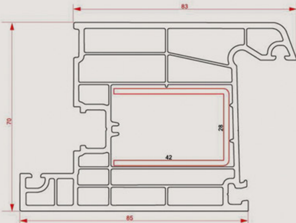
70 mm Kapi Kanat Profili 5 Odacıklı 70 mm Door Sash Profile W / 5 Chamber
