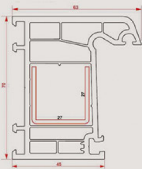
70 mm Kasa Profili 5 Odacıklı 70 mm Frame Profile W / 5 Chamber
