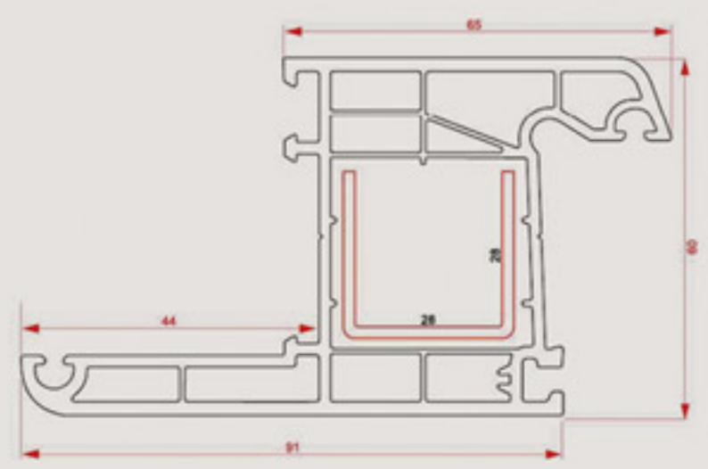
60 mm Pervazlı Kasa Profili 4 Odacıklı 60 mm Wide Frame With Border W / 4 Chamber
