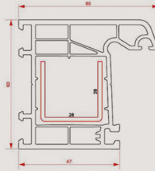
60 mm Kasa Profili 4 Odacıklı 60 mm Frame Profile W / 4 Chamber
